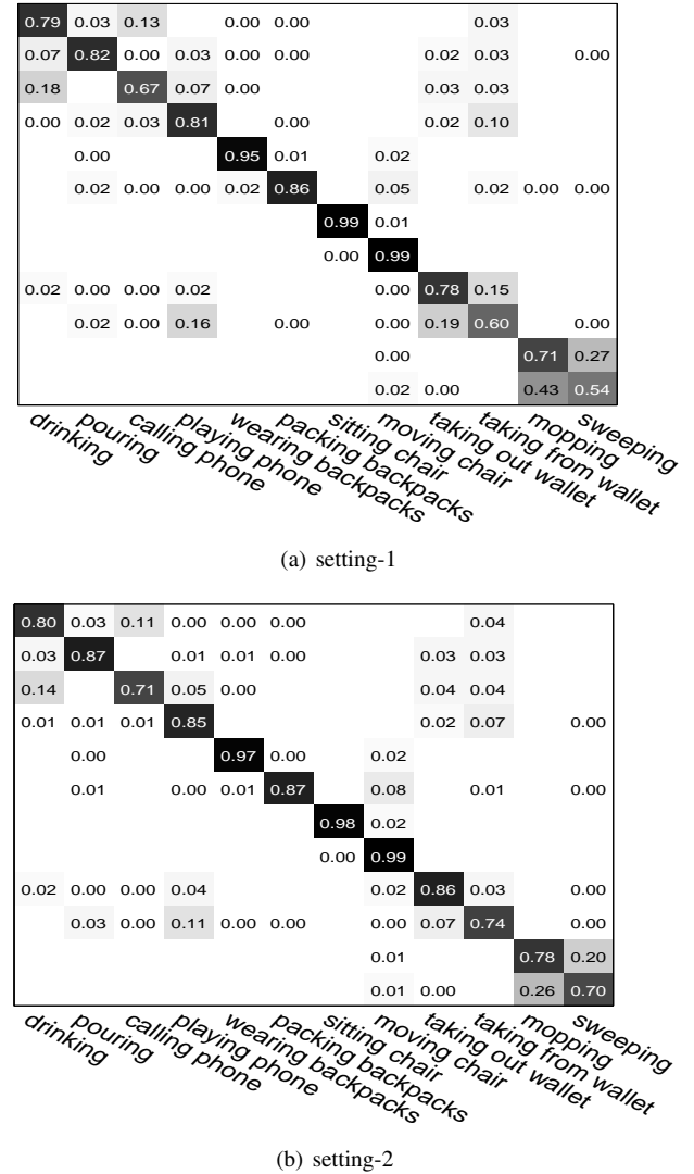
Fig. 7. Confusion matrices of JOULE on SYSU 3D HOI set.
