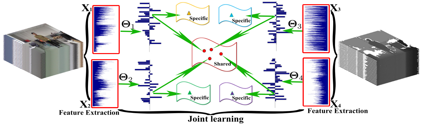
Fig. 2. A graphic illustration of our joint learning framework. In this framework, all the i-transforms (e.g. four i-transforms, \{\Theta_i\}_{i=1,2,3,4} ) shared structures and specific structures are jointly learned for the purpose of recognition on RGB and Depth channels.
